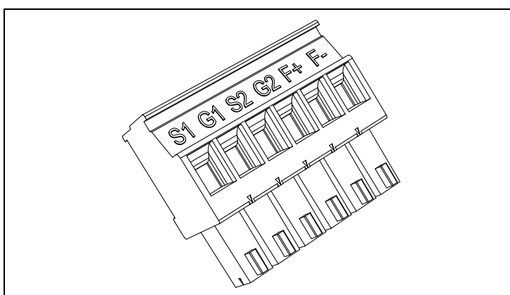
Figure 7. STO connector.
