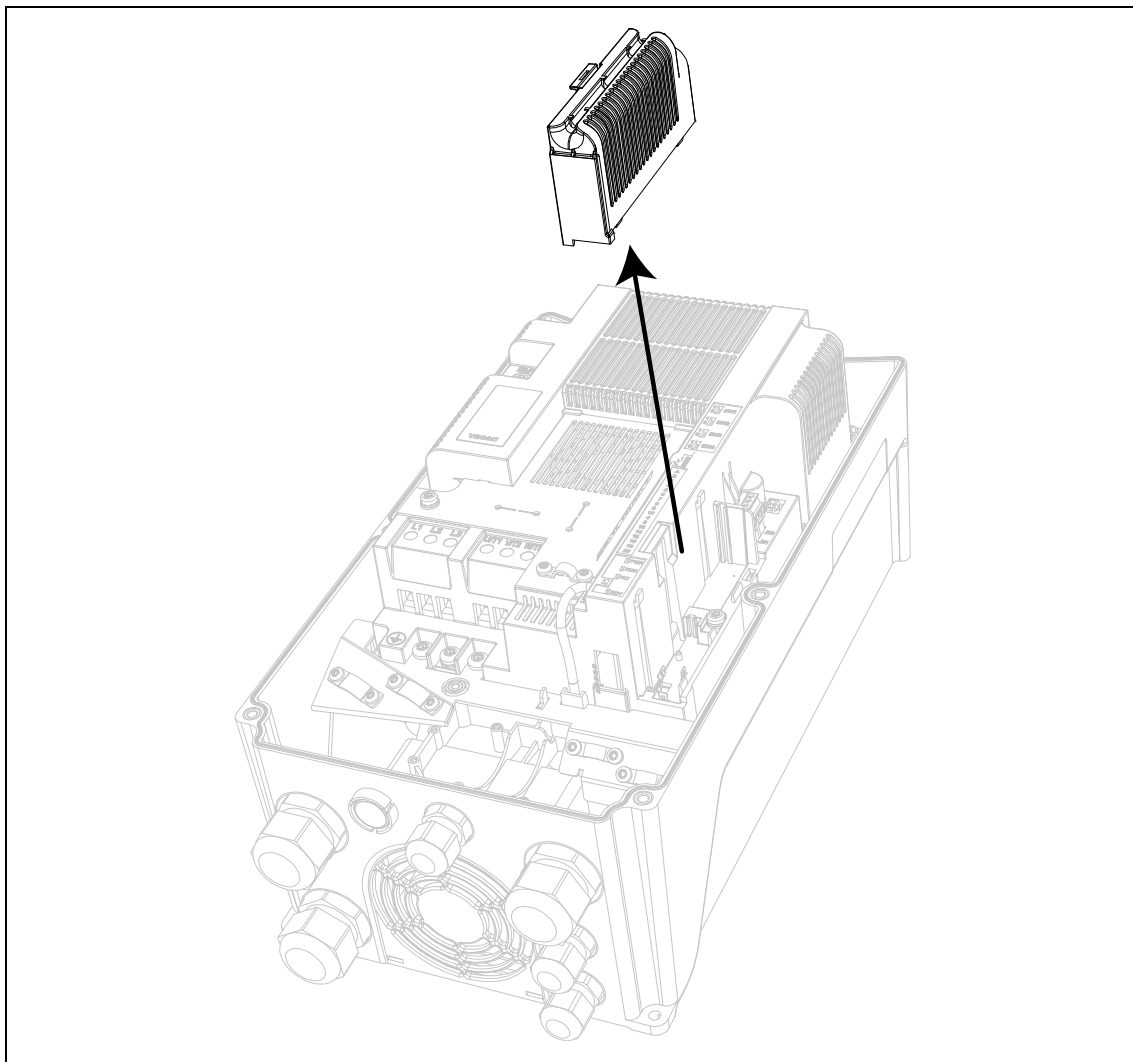
Figure 47. Removing the option slot cover.
