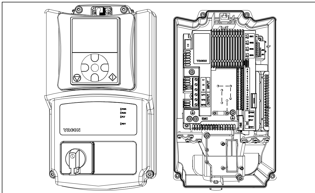
Figure 18. MU2 example: open cover.
