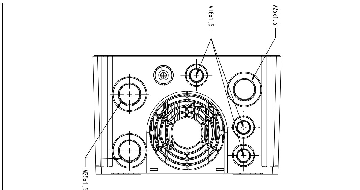
Figure 20. Cable entries, MU3.
