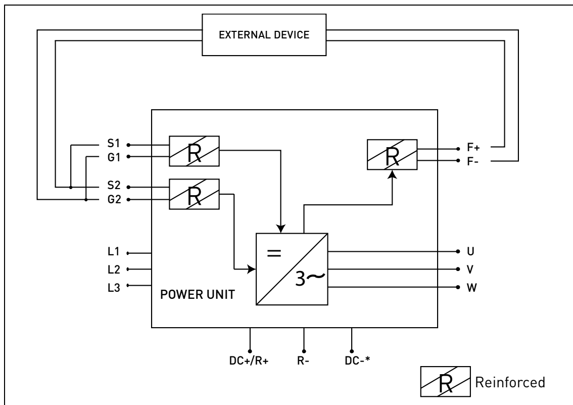
Figure 54. STO Example with automatic monitoring of the feedback and STO inputs connected in parallel. (*) Only for MU3.
