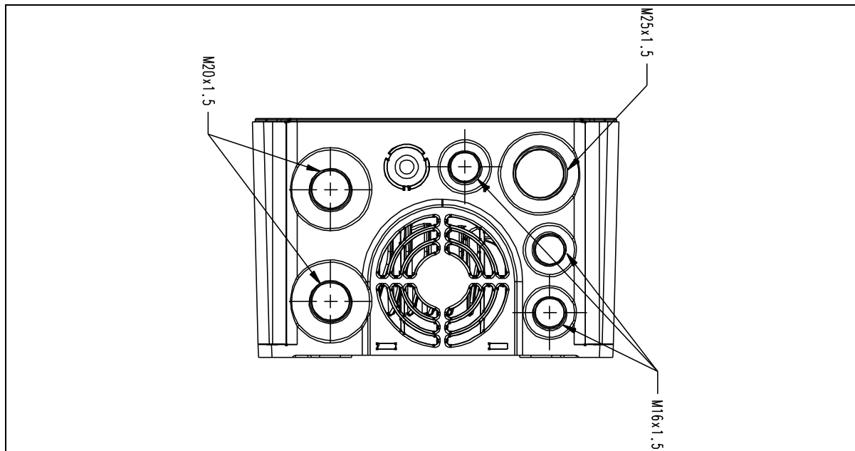
Figure 19. Cable entries, MU2.
