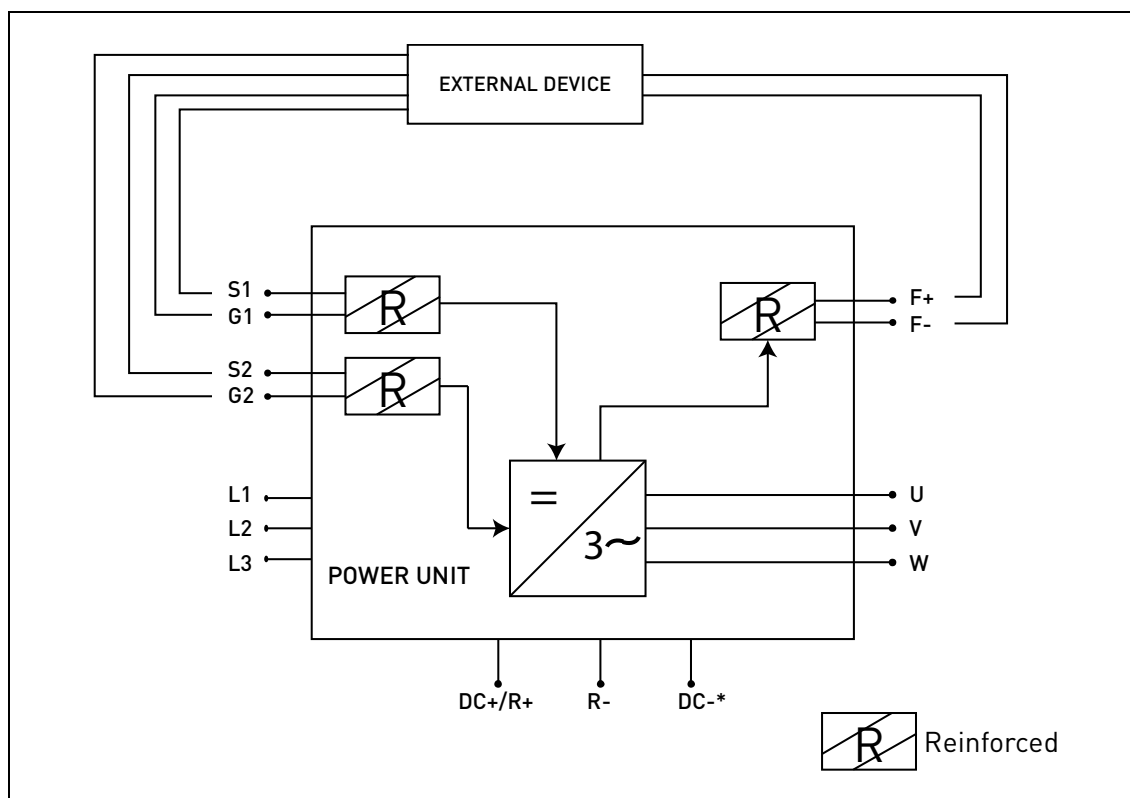
Figure 53. STO example with automatic monitoring of the feedback and both STO inputs used. (*) Only for MU3.
