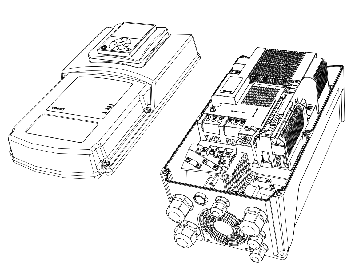
Figure 46. Opening the main cover, MU3 example.
