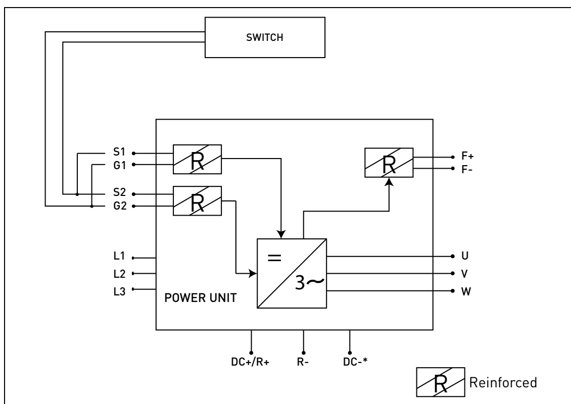
Figure 55. STO example without automatic monitoring of the feedback and STO inputs connected in parallel. (*)Only for MU3.
