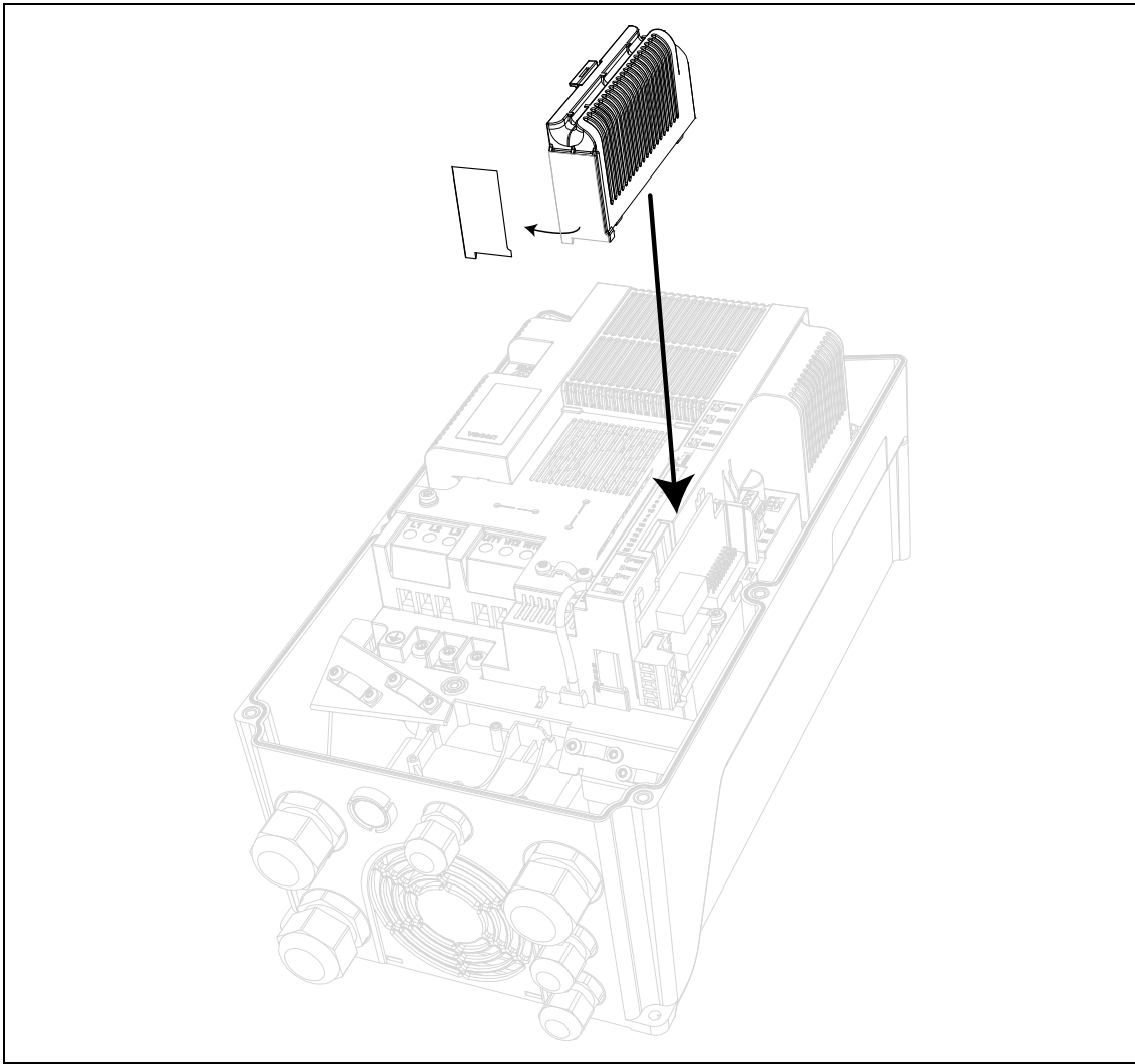
Figure 49. Mounting of option slot cover: remove the plastic opening for the option board terminals.
