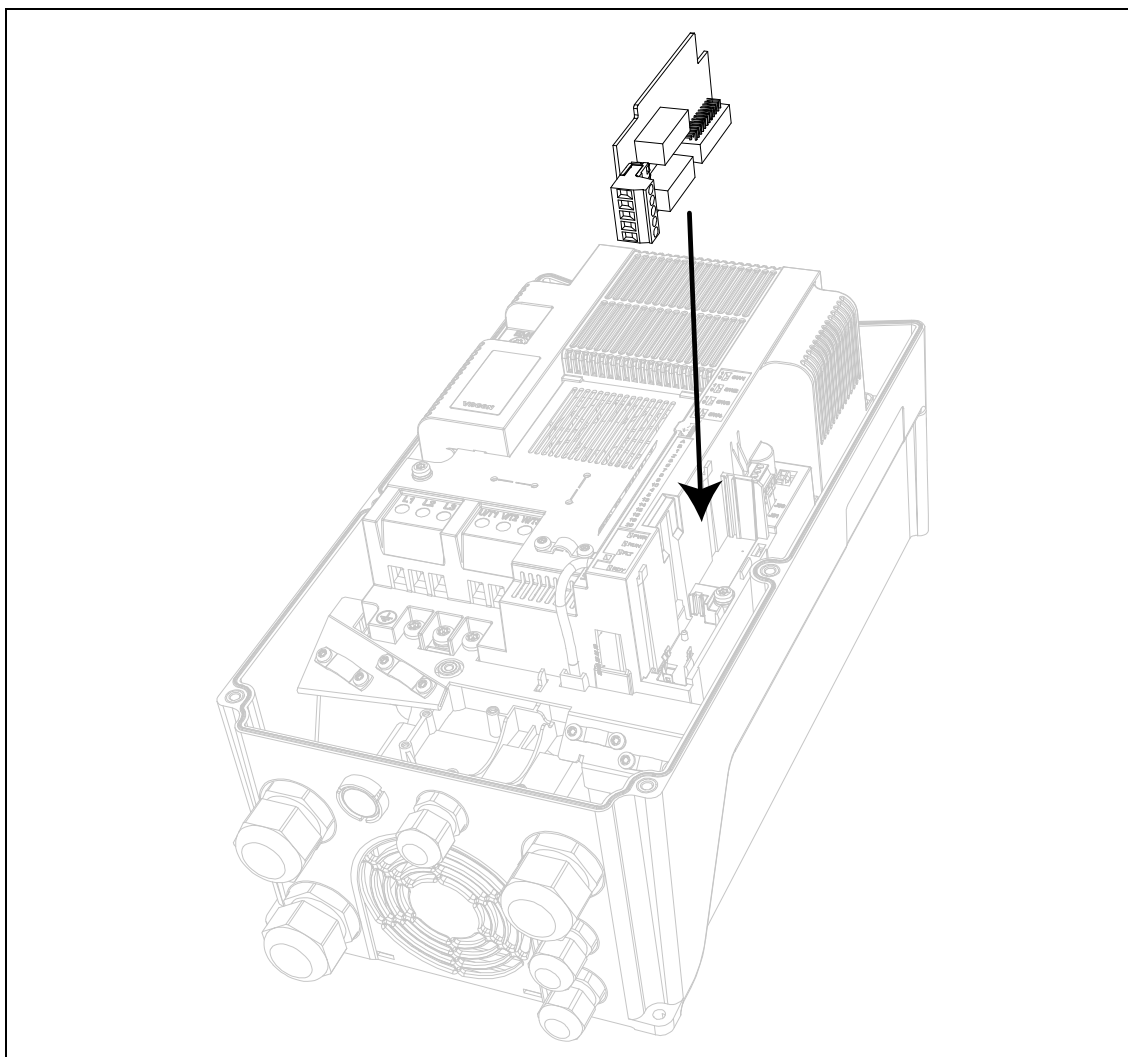
Figure 48. Option board installation.
