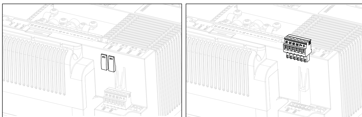
Figure 51. Removing the STO jumpers from the control unit.
