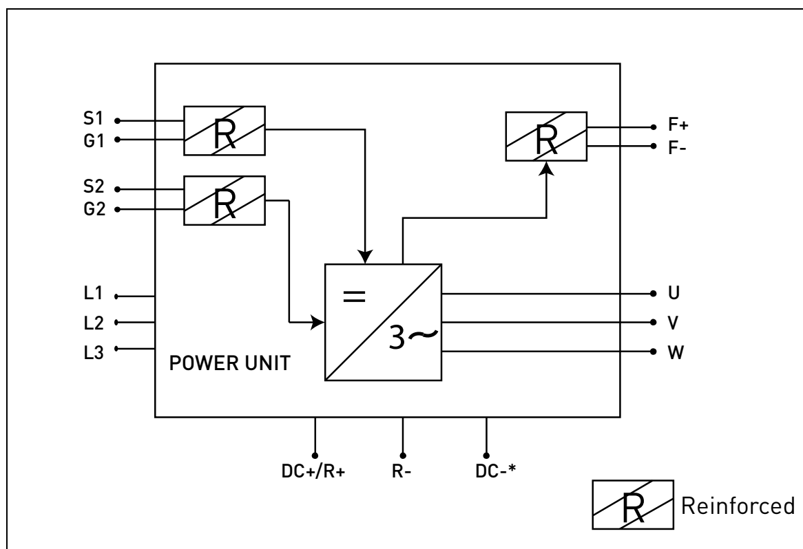
Figure 50. STO function principle. (*) Only for MU3.
